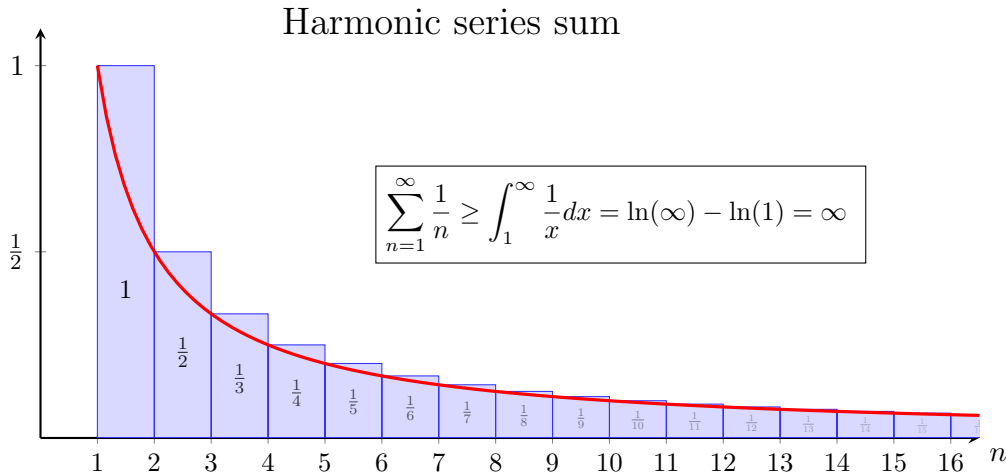
Figure 5: The harmonic series sum diverges. The sum of the areas of the blue rectangles (left) exceeds the area under the red curve (right), which diverges as x \rightarrow \infty . Thus, \sum_{n=1}^{\infty} \frac{1}{n} = \infty . This fact will be used to show that the expected time to extinction in the critical Galton–Watson process is infinite.
