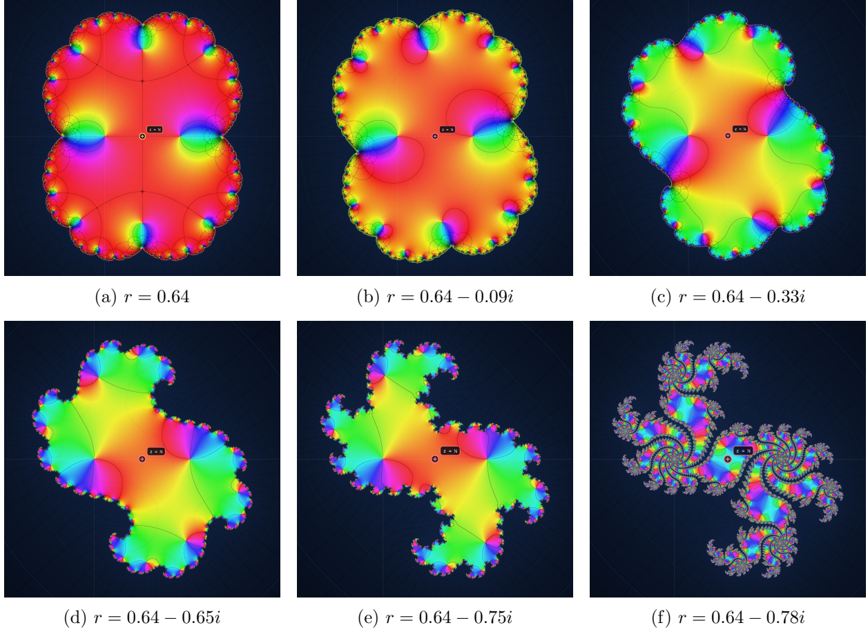
Figure 8: Continuation from the real branching slice at \operatorname{Re} r = 0.64 . Panel (a) is the branching case p = 0.32 , with A(p) = 0.335521 and 1/A(p) = 2.980439 . In (b)–(e), |r| is 0.646, 0.720, 0.912 and 0.986: the Koenigs coordinate persists, but r/2 is no longer a probability. In (f), |r| \approx 1.009 and the attracting chart no longer applies. The marked point is z = \frac{1}{2} throughout.
