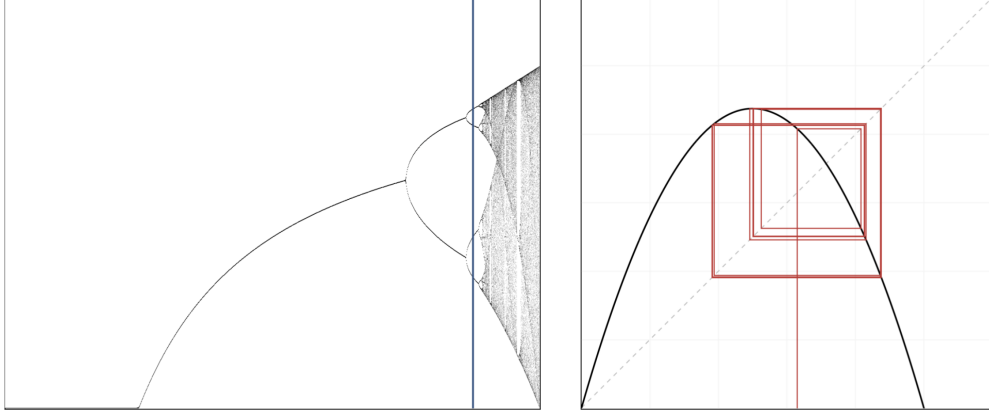
Figure 3: Aside, not used in the argument. Phase diagram of the logistic map that shows the period doubling of stable states, ultimately resulting in chaotic behaviour. Blue sample line on the left at r = 3.5255 , right plot shows a trajectory of the map with the same value of r . The subcritical branching window is r = 2p \in (0, 1) , at the far left of this diagram, where the only attractor is the fixed point at the origin.
