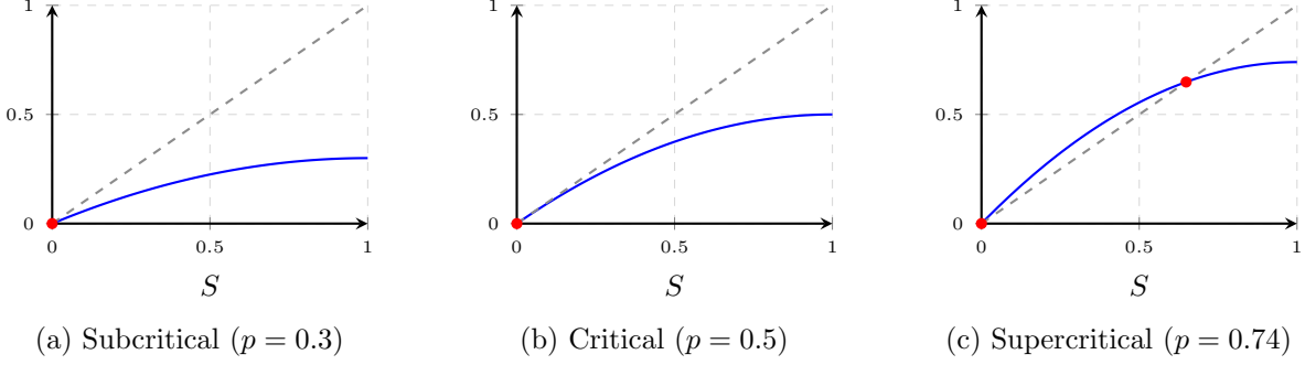
Figure 1: Fixed points of the survival recursion S \mapsto 2pS - pS^2 . Each panel shows the map (blue) against the diagonal (dashed), with fixed points marked in red. Below and at criticality the only fixed point in [0, 1] is the origin; for p > \frac{1}{2} a stable positive root S_\infty = (2p - 1)/p separates from it (at p = 0.74 , this is approximately 0.649).
