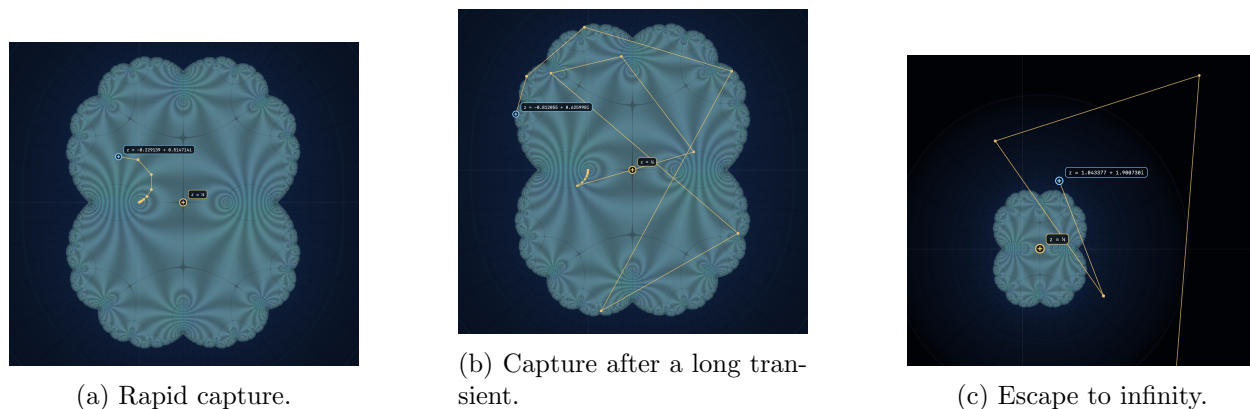
Figure 6: Orbit fates for f_r(z) = rz(1 - z) at r = 0.64 ( p = 0.32 ). The seeds z = -0.229139 + 0.514714i , z = -0.812055 + 0.625998i and z = 1.043377 + 1.900730i in (a)–(c) give, respectively, rapid capture, capture after a long transient and escape. The first two therefore lie in the same attracting basin.
