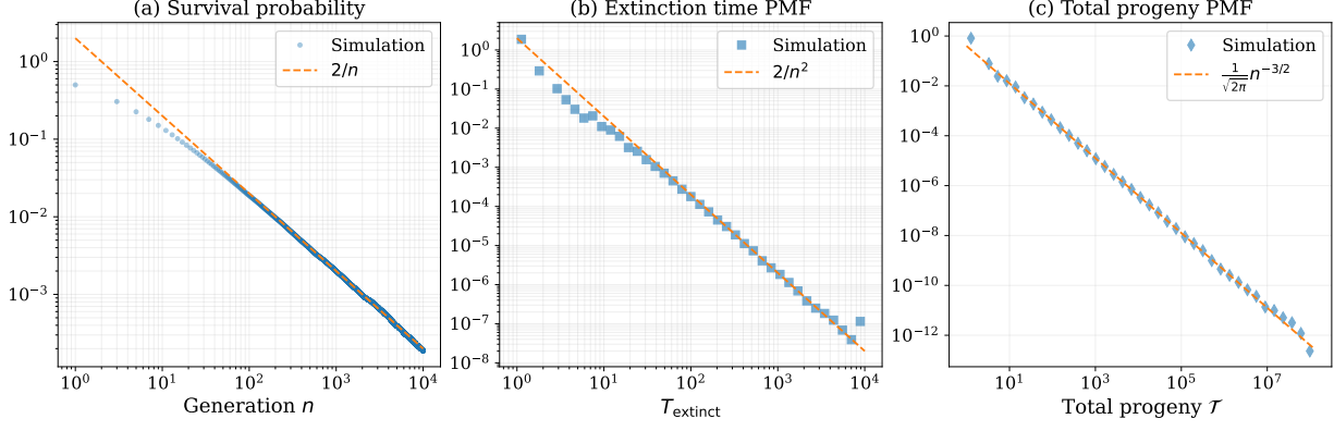
Figure 4: Power-law behaviour in a critical Galton–Watson branching process ( p = 0.5 ). (a) Survival probability S_n = \mathbb{P}(Z_n > 0) , showing the late generation asymptotic scaling S_n \sim 2/n . (b) Probability mass function of the extinction time T_{\text{extinct}} = \inf\{n : Z_n = 0\} , exhibiting a heavy tail \mathbb{P}(T_{\text{extinct}} = n) \sim 2/n^2 . (c) Probability mass function of the total progeny \mathcal{T} = \sum_{k \geq 0} Z_k , displaying the classical critical branching asymptotic \mathbb{P}(\mathcal{T} = n) \sim n^{-3/2} . ( 10^6 realisations).
